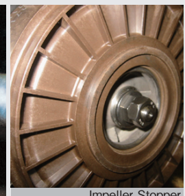
Impeller Stopper
