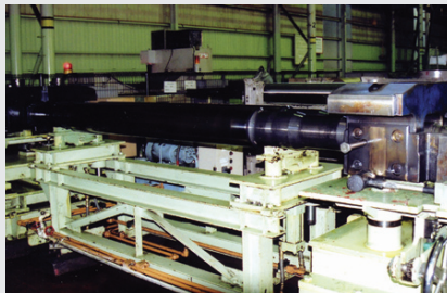
Steel Making Machinery (Straightening Roll Stopper)
