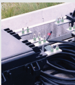
Impedance Bond
