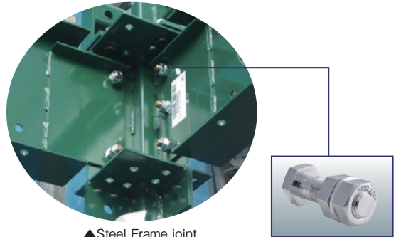
▲Steel Frame joint
